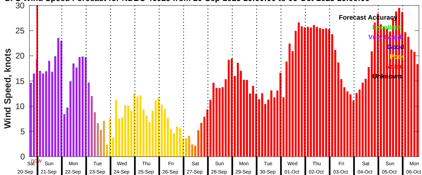
GFS Wind Speed Forecast for NDBC 46028 from 20-Sep-2025 16:00:00 to 06-Oct-2025 16:00:00
