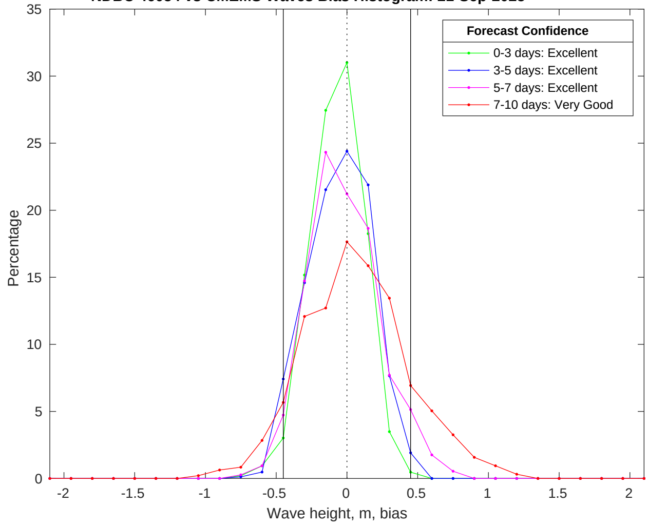
NDBC 46054 vs CMEMS Waves Bias Histogram: 21-Sep-2025
