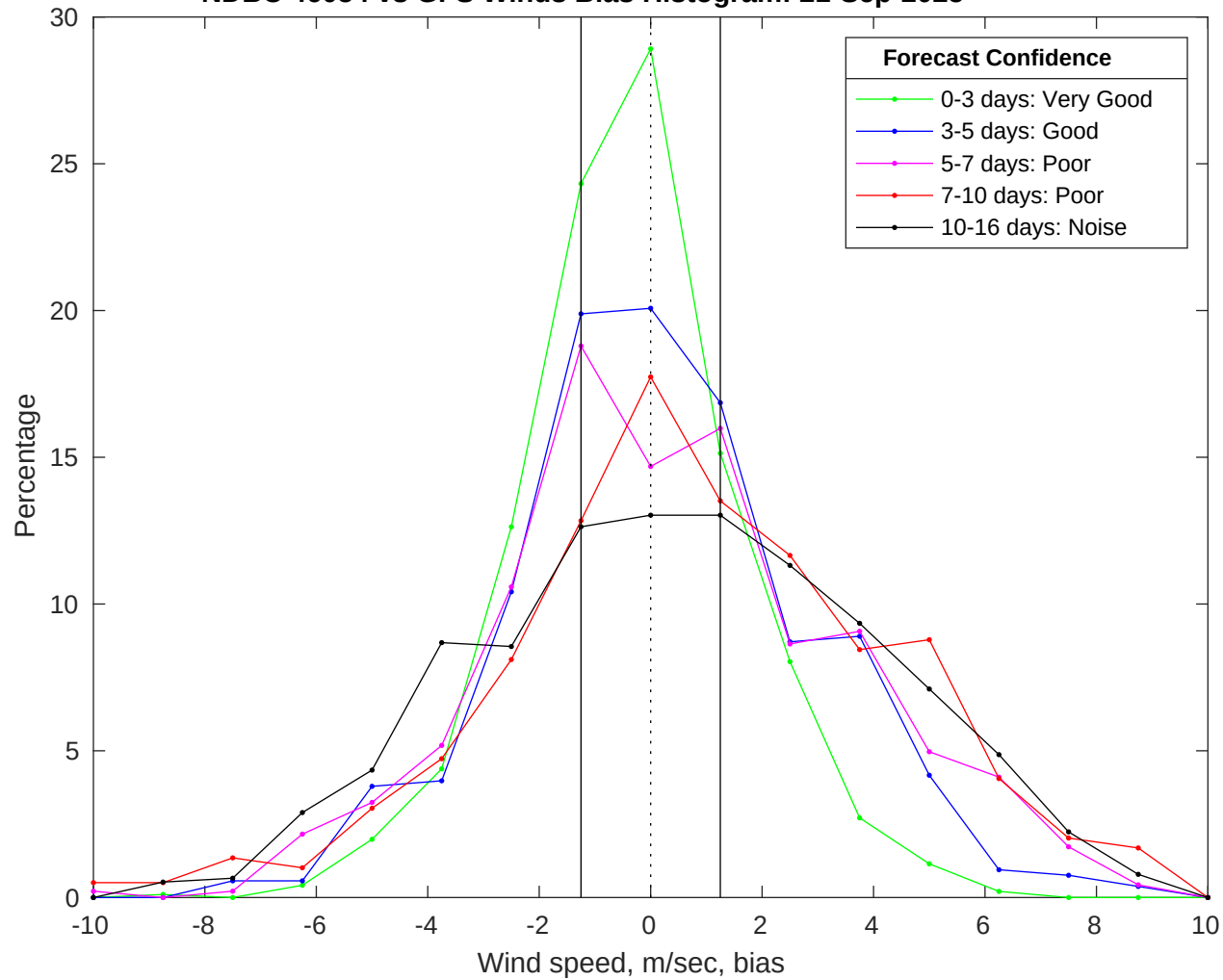
NDBC 46054 vs GFS Winds Bias Histogram: 21-Sep-2025
