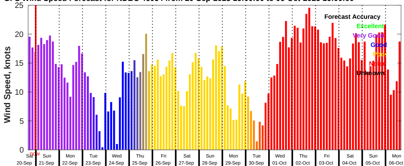
GFS Wind Speed Forecast for NDBC 46054 from 20-Sep-2025 16:00:00 to 06-Oct-2025 16:00:00
