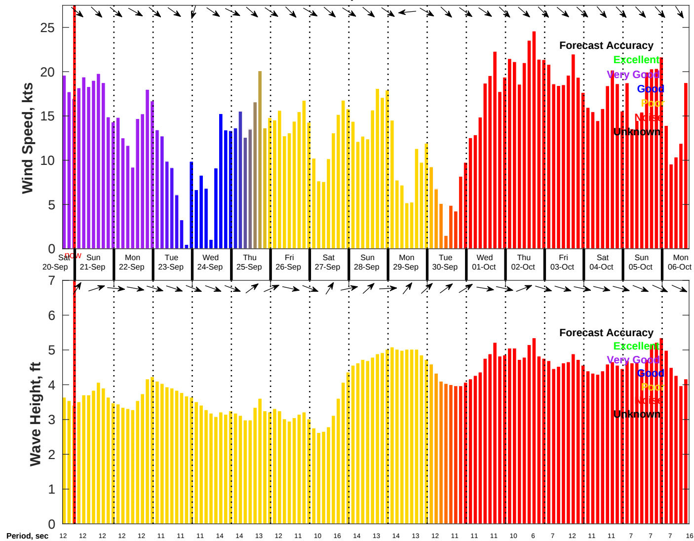
Wind & Wave Forecast for NDBC 46054 from 20-Sep-2025 16:00:00 to 06-Oct-2025 16:00:00
