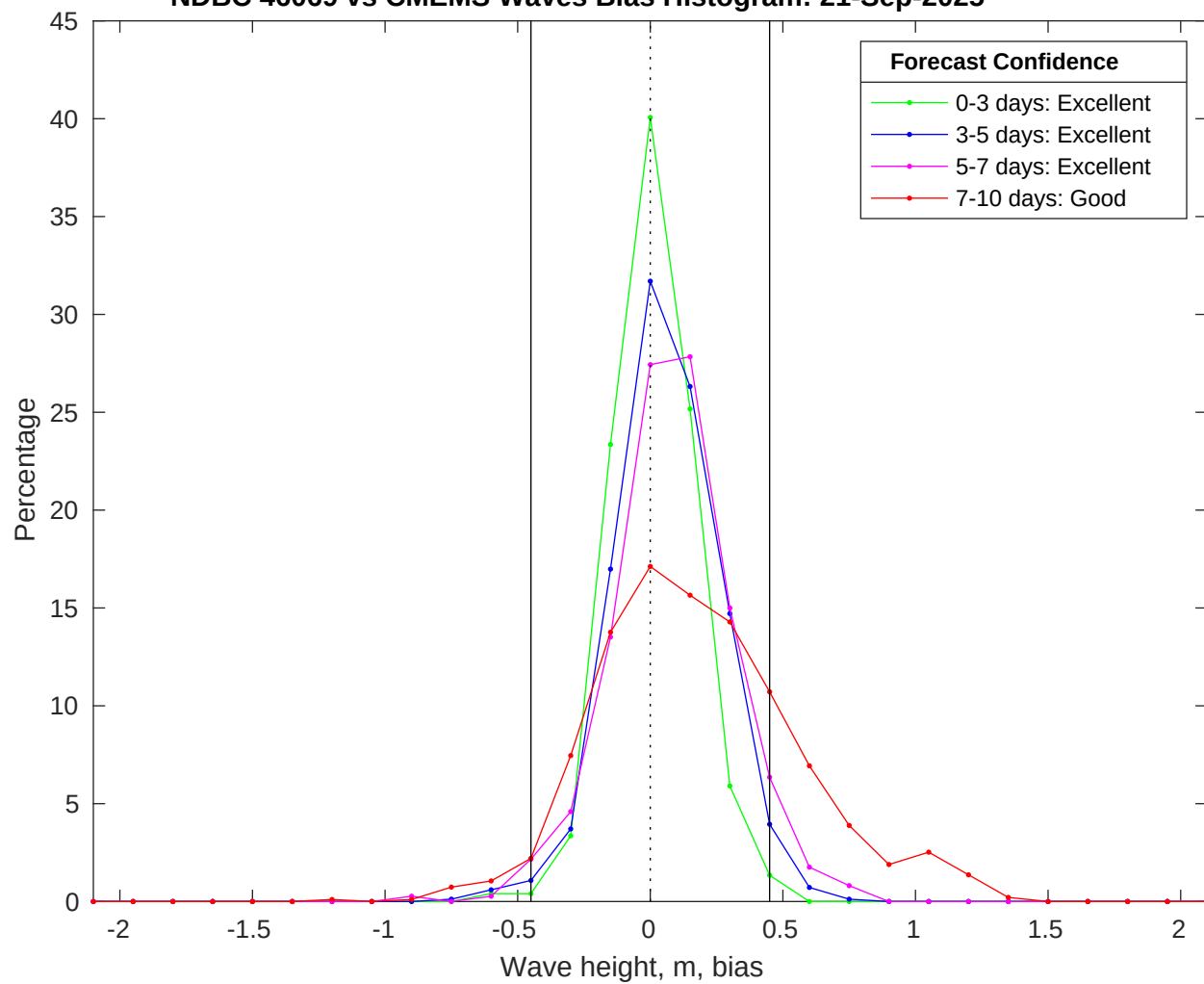
NDBC 46069 vs CMEMS Waves Bias Histogram: 21-Sep-2025
