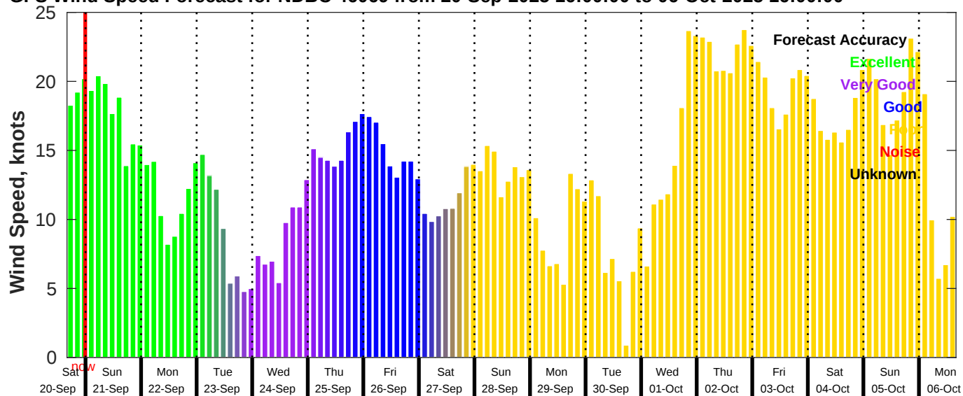
GFS Wind Speed Forecast for NDBC 46069 from 20-Sep-2025 16:00:00 to 06-Oct-2025 16:00:00
