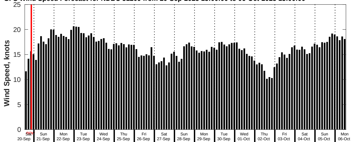
GFS Wind Speed Forecast for NDBC 51209 from 20-Sep-2025 13:00:00 to 06-Oct-2025 13:00:00
