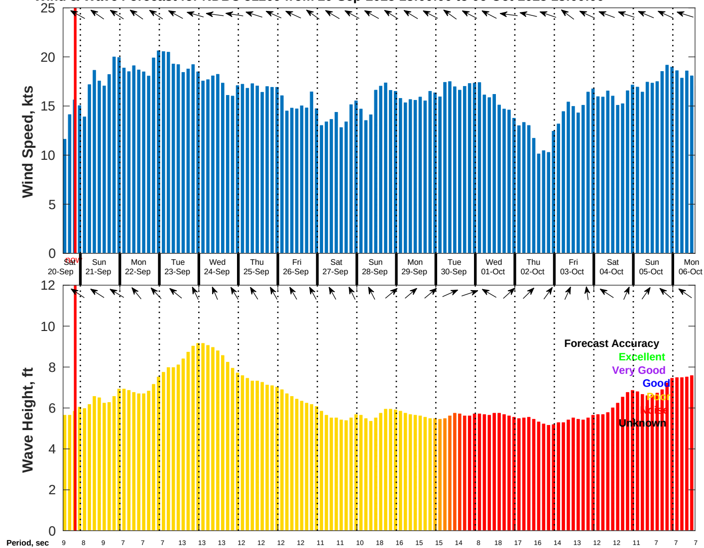
Wind & Wave Forecast for NDBC 51209 from 20-Sep-2025 13:00:00 to 06-Oct-2025 13:00:00
