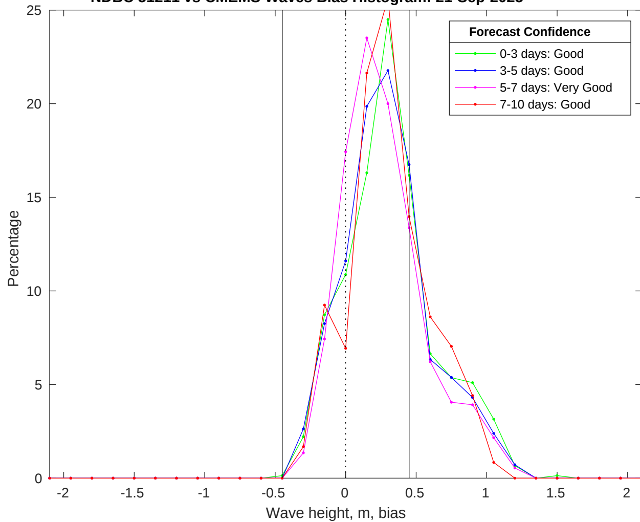
NDBC 51211 vs CMEMS Waves Bias Histogram: 21-Sep-2025
