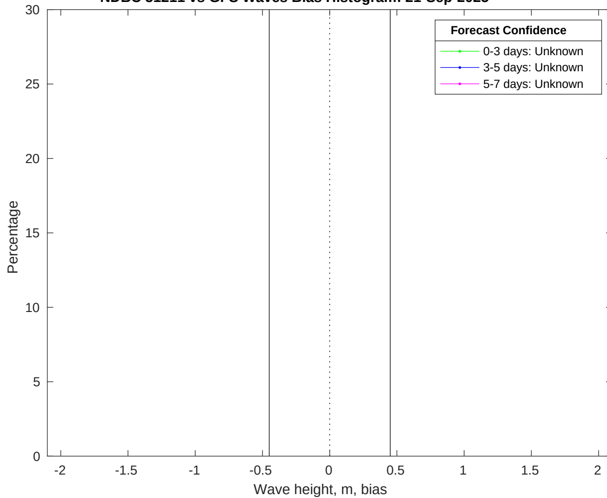
NDBC 51211 vs GFS Waves Bias Histogram: 21-Sep-2025
