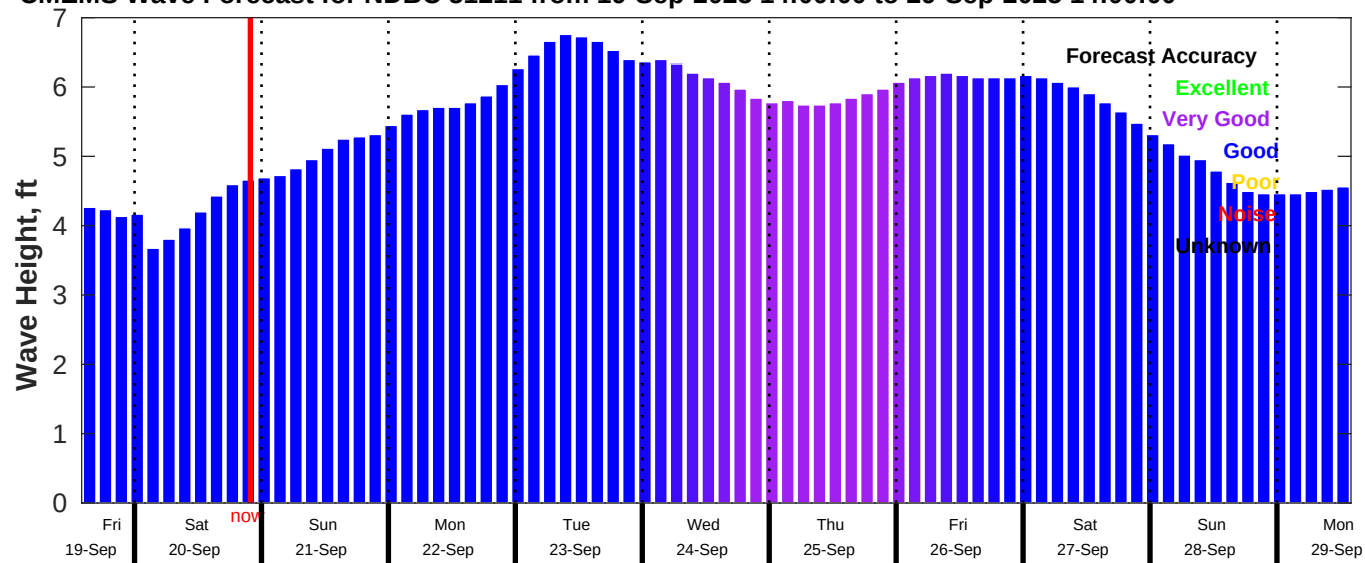
CMEMS Wave Forecast for NDBC 51211 from 19-Sep-2025 14:00:00 to 29-Sep-2025 14:00:00
