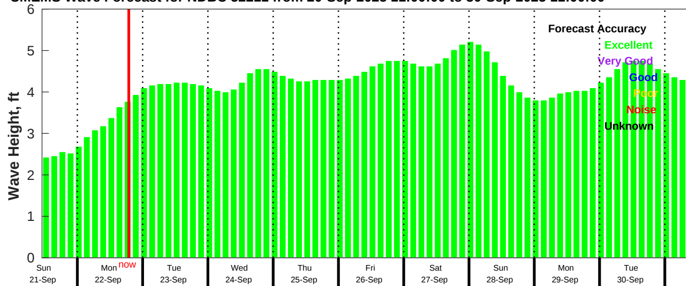
CMEMS Wave Forecast for NDBC 52211 from 20-Sep-2025 11:00:00 to 30-Sep-2025 11:00:00
