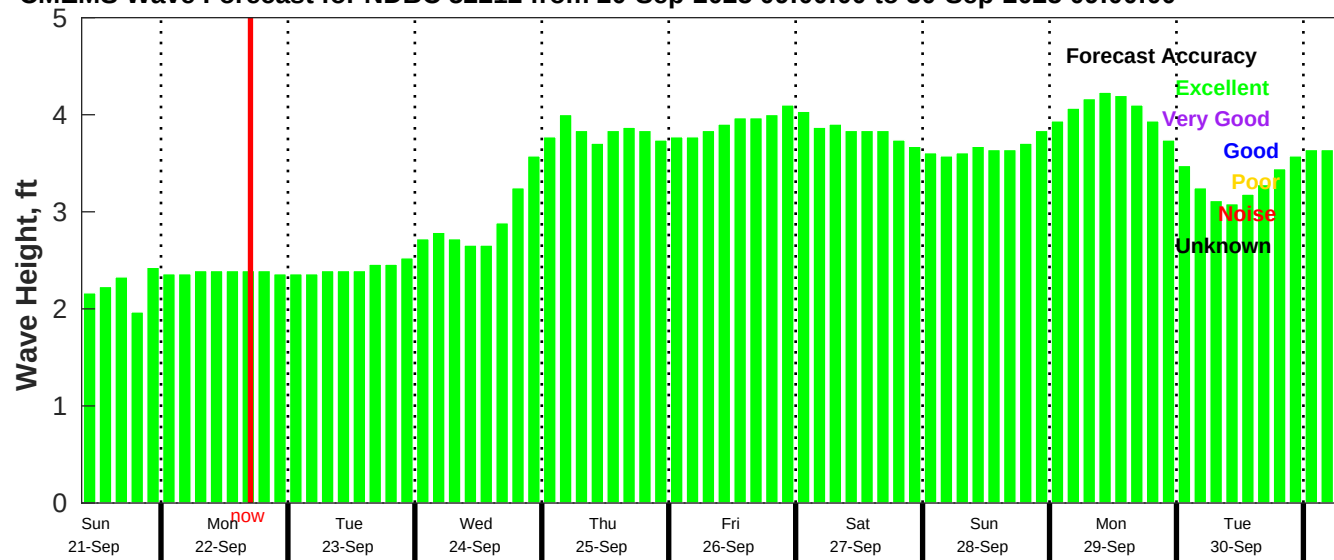
CMEMS Wave Forecast for NDBC 52212 from 20-Sep-2025 09:00:00 to 30-Sep-2025 09:00:00
