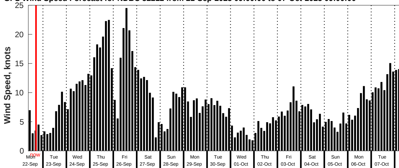
GFS Wind Speed Forecast for NDBC 52212 from 21-Sep-2025 09:00:00 to 07-Oct-2025 09:00:00
