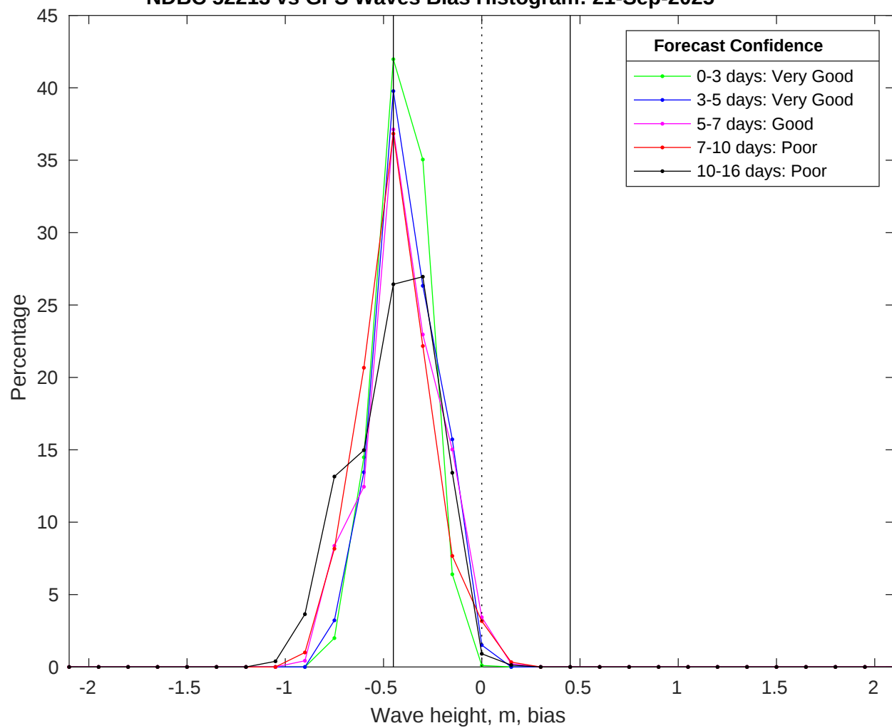
NDBC 52213 vs GFS Waves Bias Histogram: 21-Sep-2025
