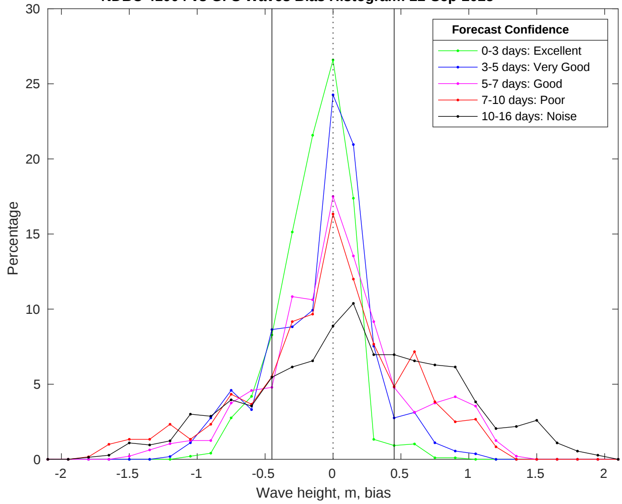
NDBC 41004 vs GFS Waves Bias Histogram: 22-Sep-2025
