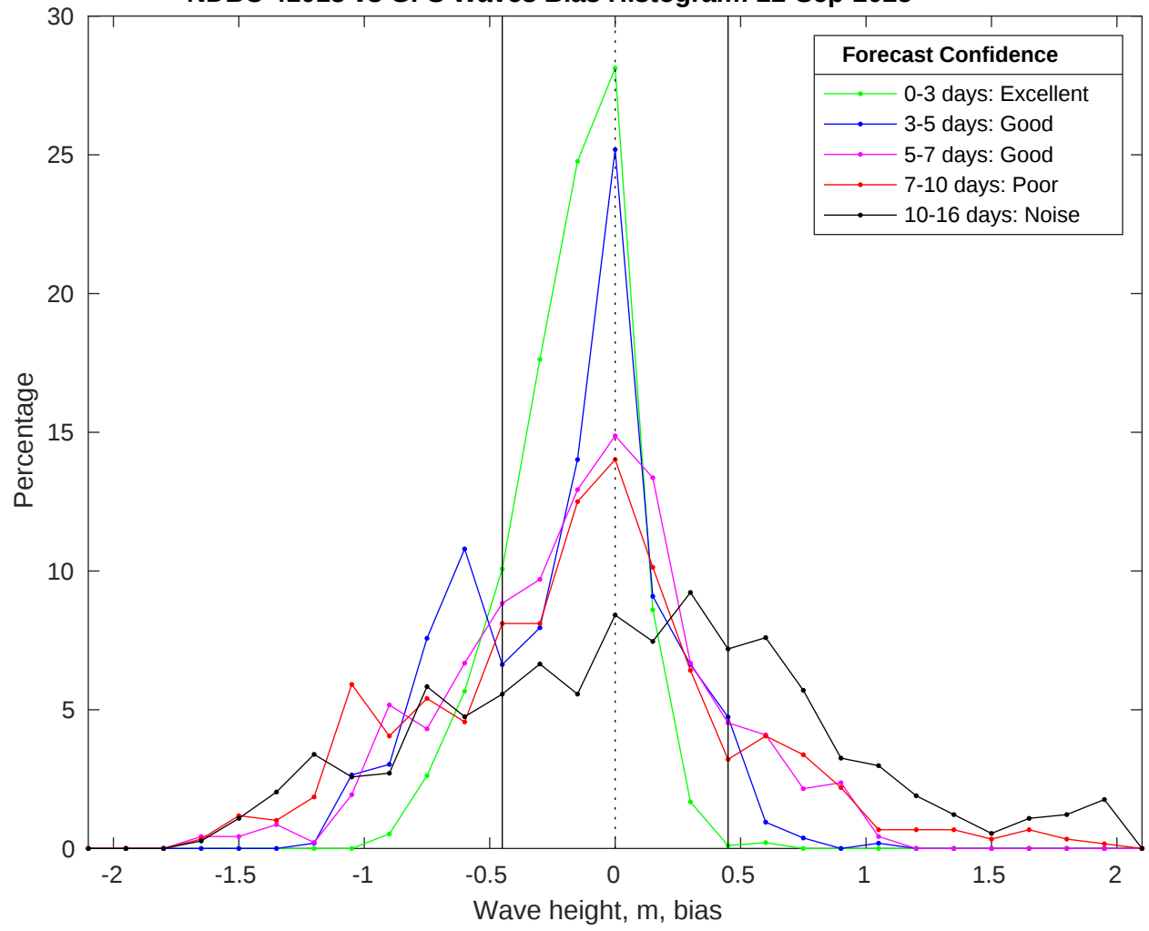
NDBC 41013 vs GFS Waves Bias Histogram: 22-Sep-2025
