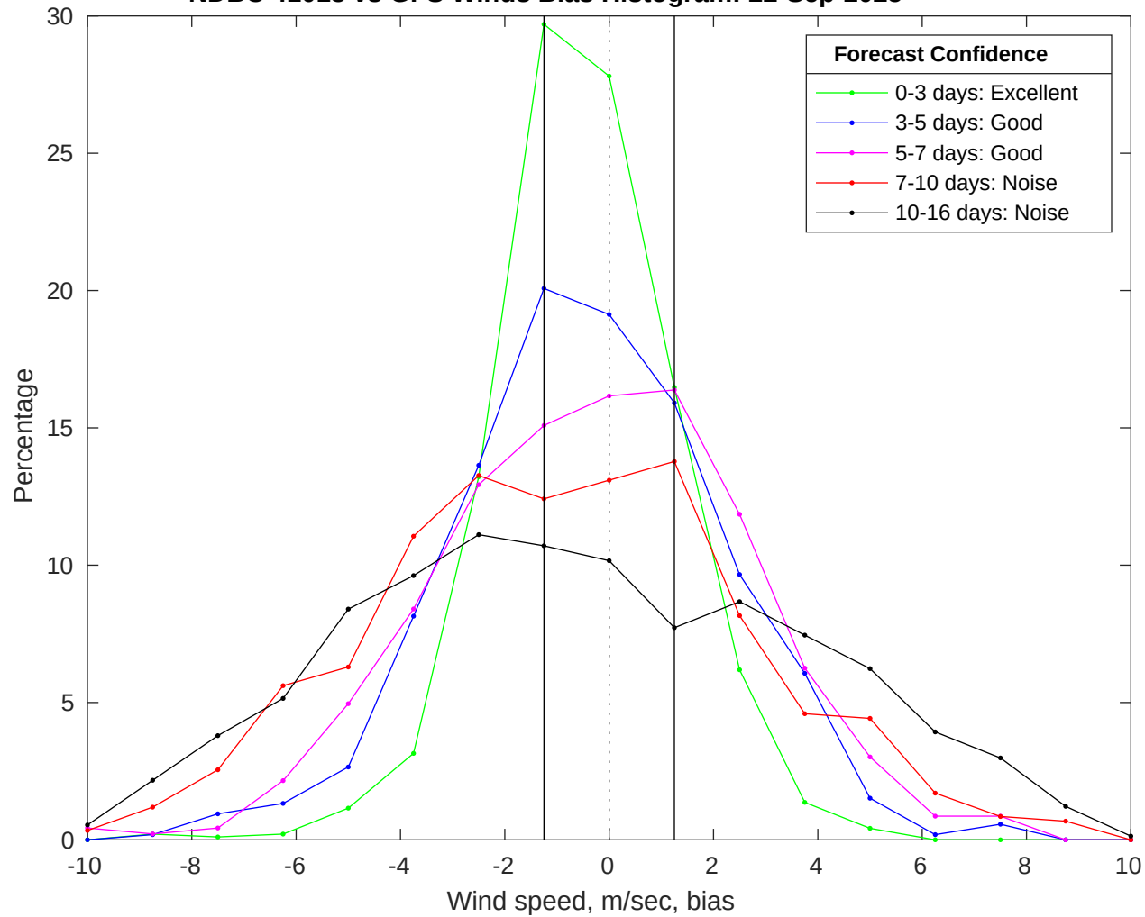
NDBC 41013 vs GFS Winds Bias Histogram: 22-Sep-2025
