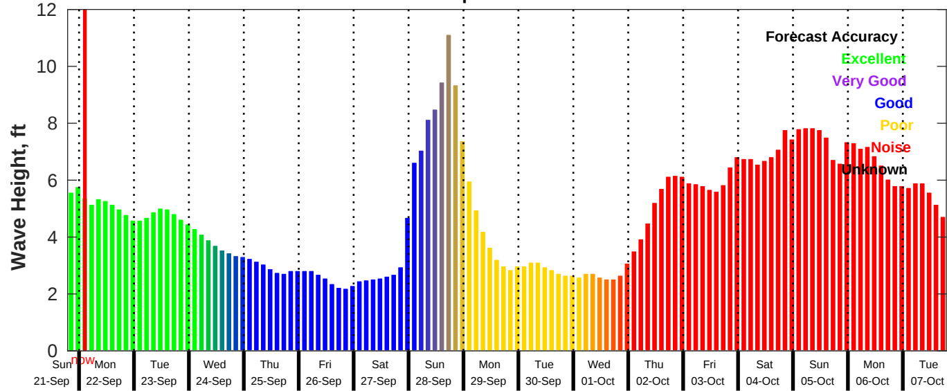
GFS Wave Forecast for NDBC 41013 from 21-Sep-2025 19:00:00 to 07-Oct-2025 19:00:00
