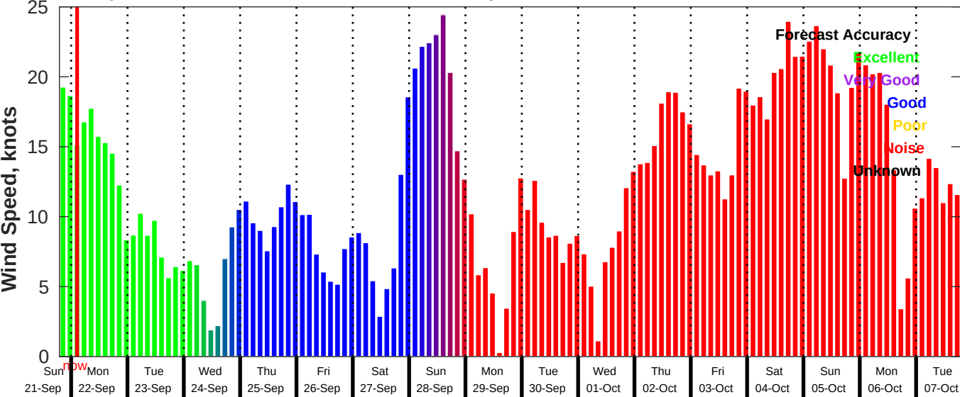
GFS Wind Speed Forecast for NDBC 41013 from 21-Sep-2025 19:00:00 to 07-Oct-2025 19:00:00
