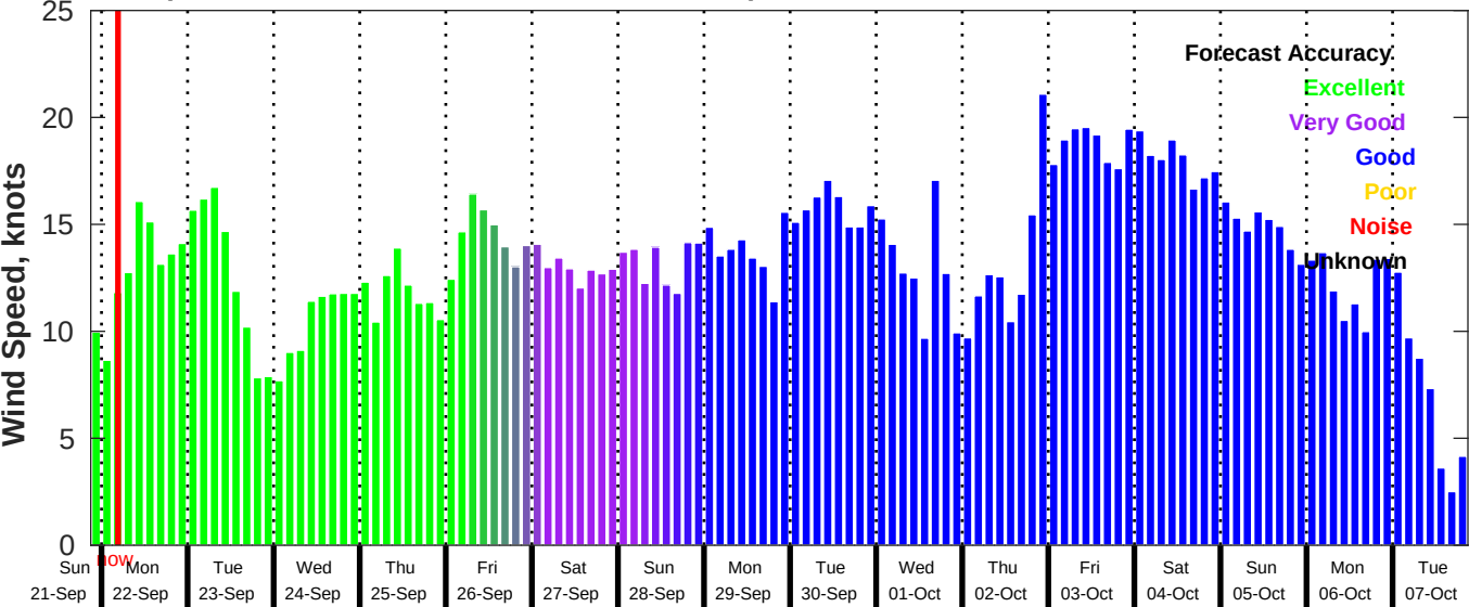
GFS Wind Speed Forecast for NDBC 41040 from 21-Sep-2025 21:00:00 to 07-Oct-2025 21:00:00
