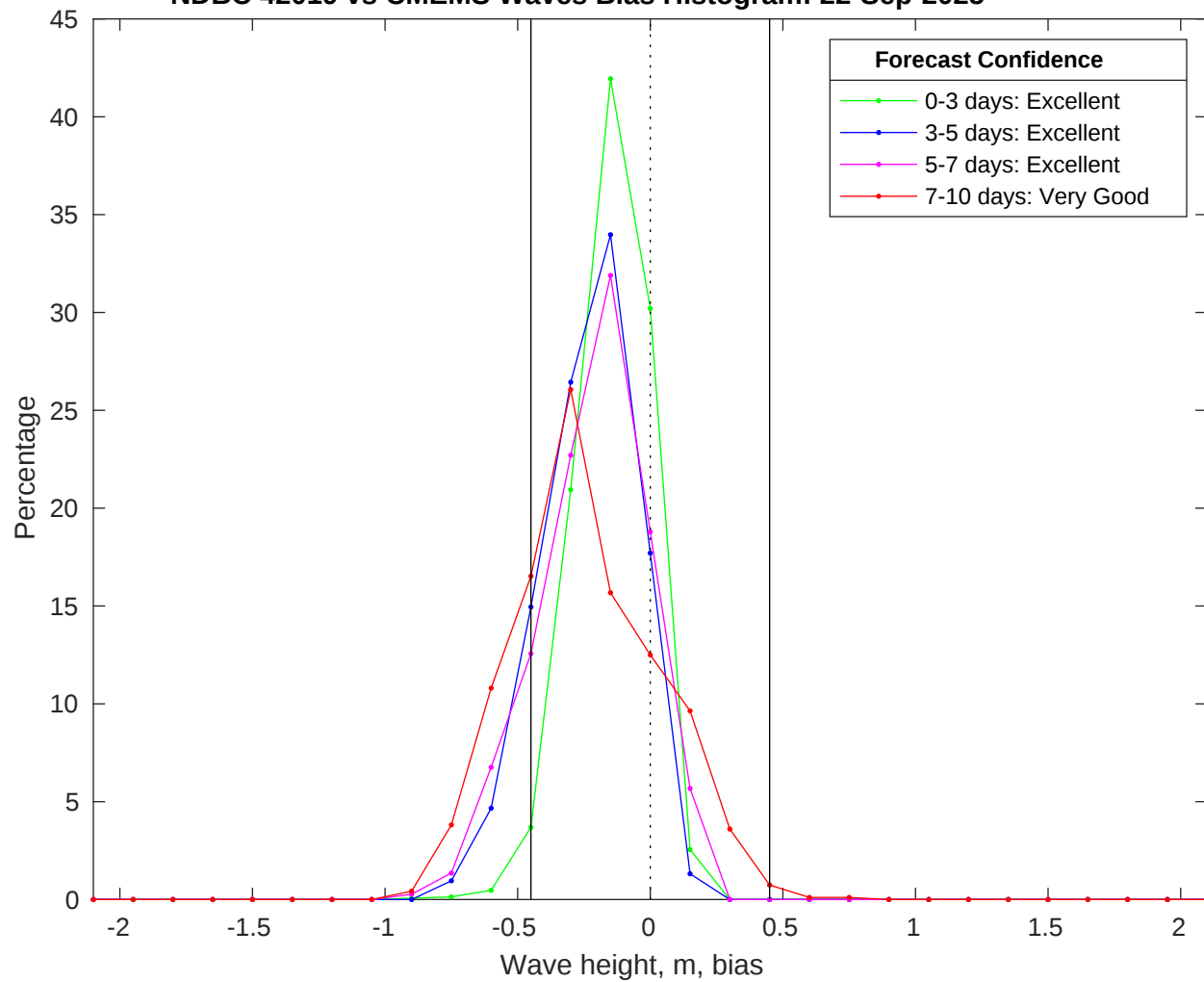
NDBC 42019 vs CMEMS Waves Bias Histogram: 22-Sep-2025
