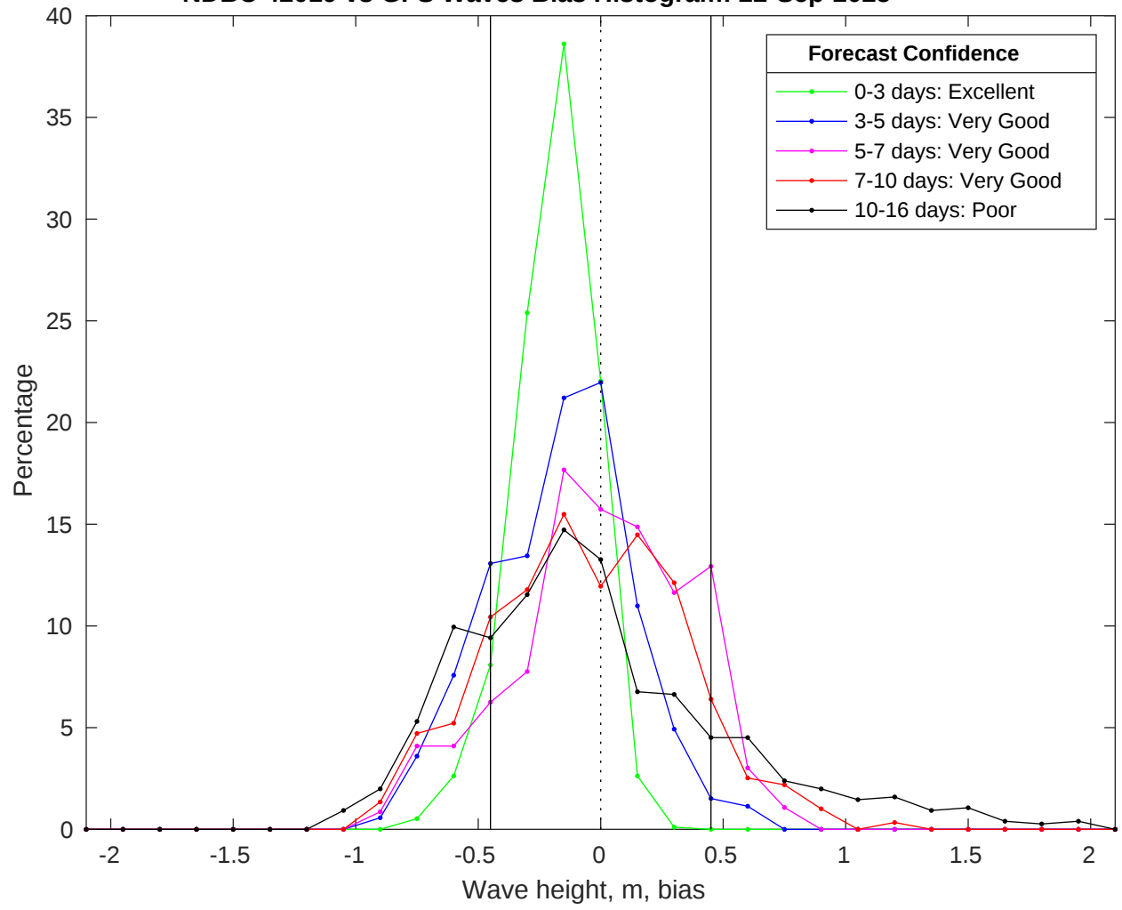
NDBC 42019 vs GFS Waves Bias Histogram: 22-Sep-2025
