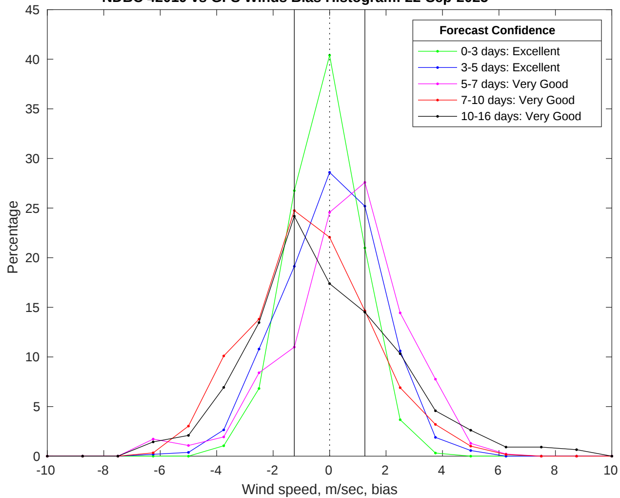
NDBC 42019 vs GFS Winds Bias Histogram: 22-Sep-2025
