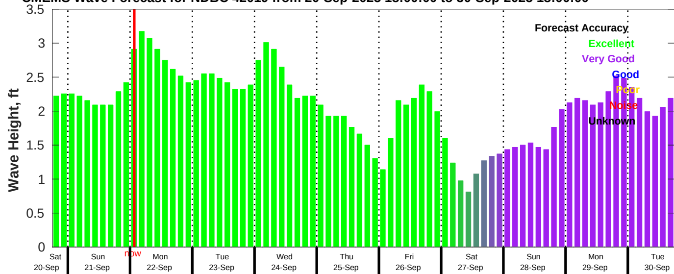
CMEMS Wave Forecast for NDBC 42019 from 20-Sep-2025 18:00:00 to 30-Sep-2025 18:00:00
