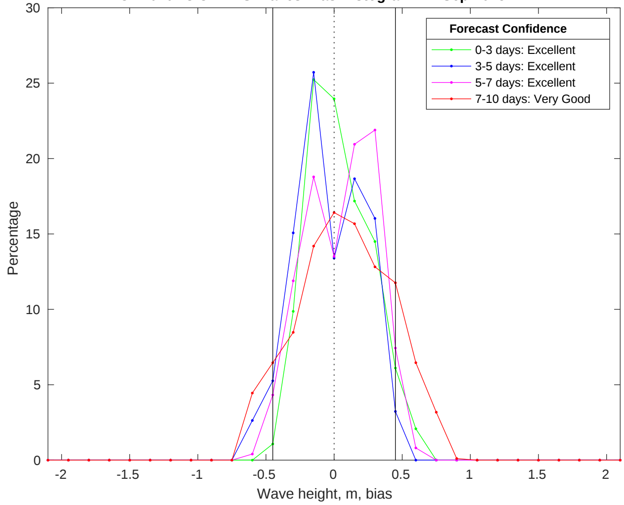
NDBC 42020 vs CMEMS Waves Bias Histogram: 22-Sep-2025
