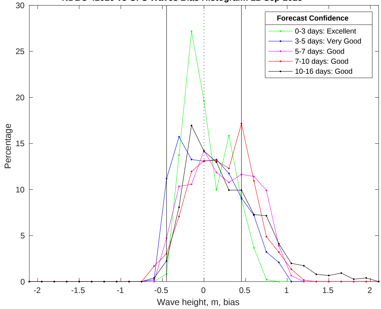
NDBC 42020 vs GFS Waves Bias Histogram: 22-Sep-2025
