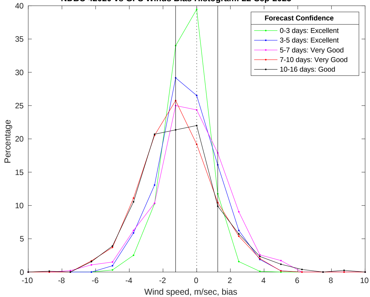
NDBC 42020 vs GFS Winds Bias Histogram: 22-Sep-2025
