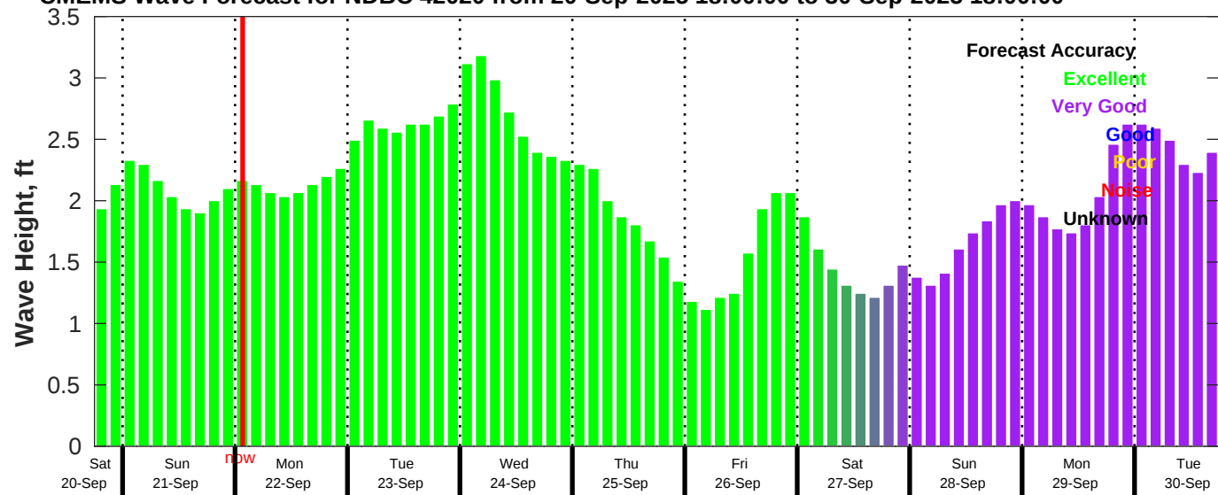
CMEMS Wave Forecast for NDBC 42020 from 20-Sep-2025 18:00:00 to 30-Sep-2025 18:00:00
