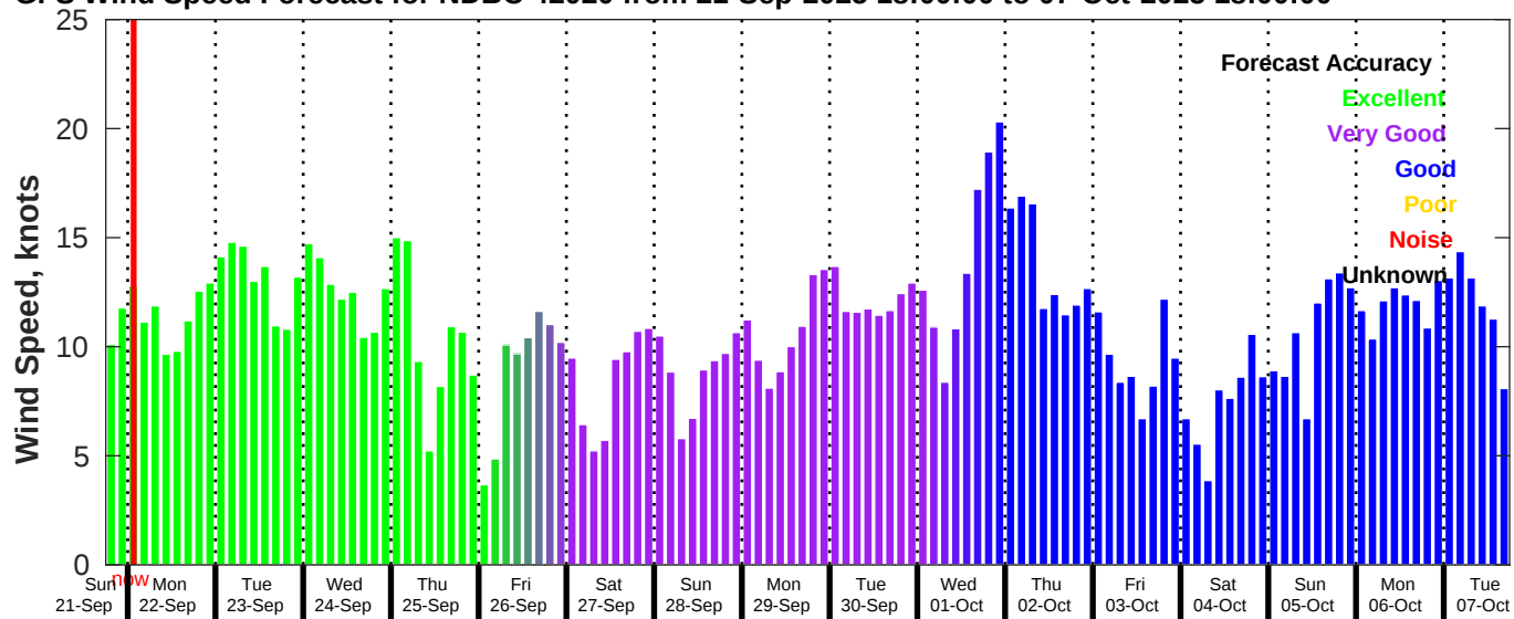
GFS Wind Speed Forecast for NDBC 42020 from 21-Sep-2025 18:00:00 to 07-Oct-2025 18:00:00
