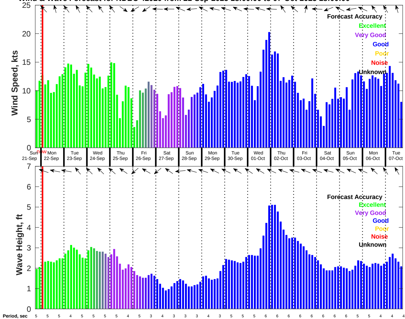
Wind & Wave Forecast for NDBC 42020 from 21-Sep-2025 18:00:00 to 07-Oct-2025 18:00:00
