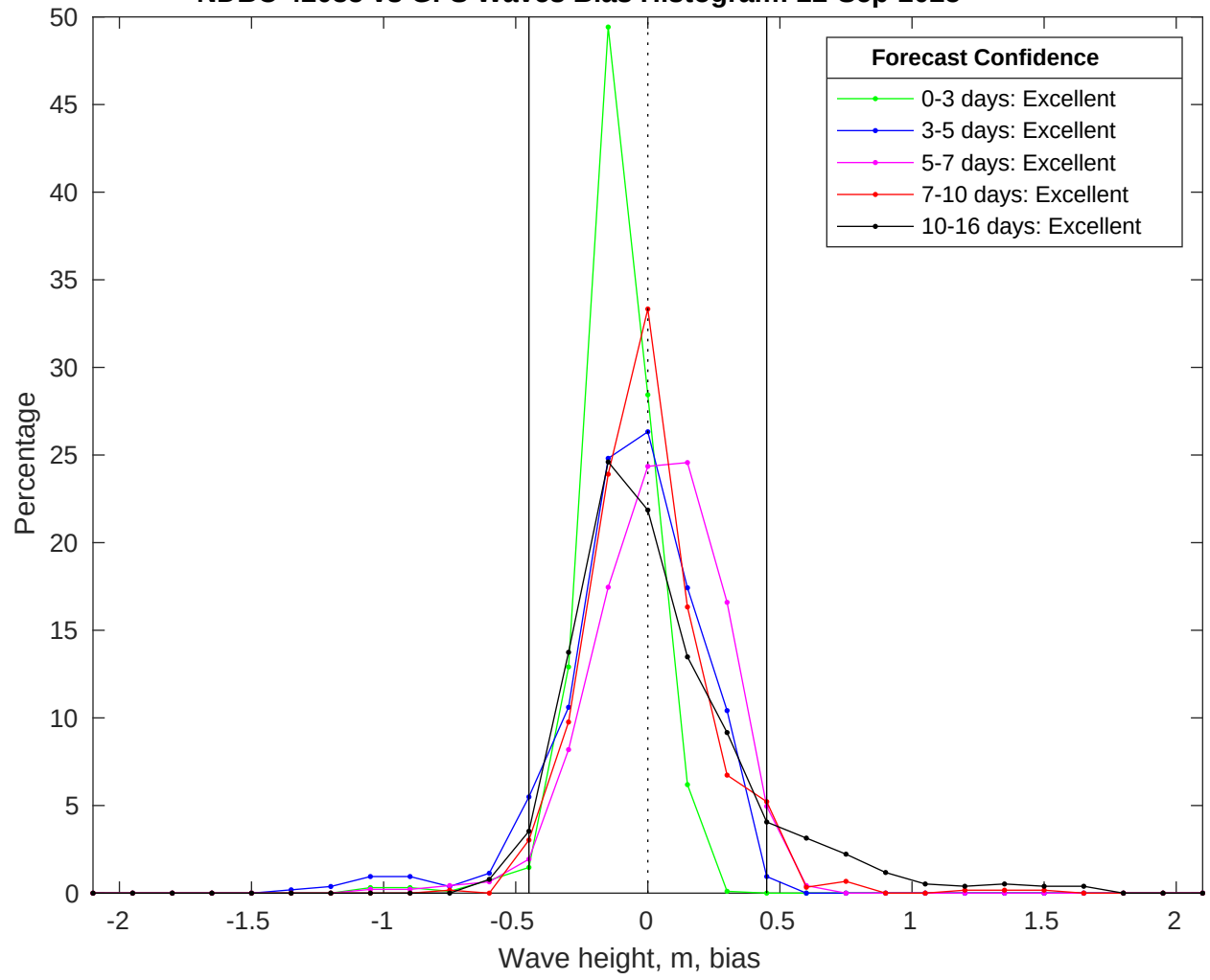
NDBC 42035 vs GFS Waves Bias Histogram: 22-Sep-2025
