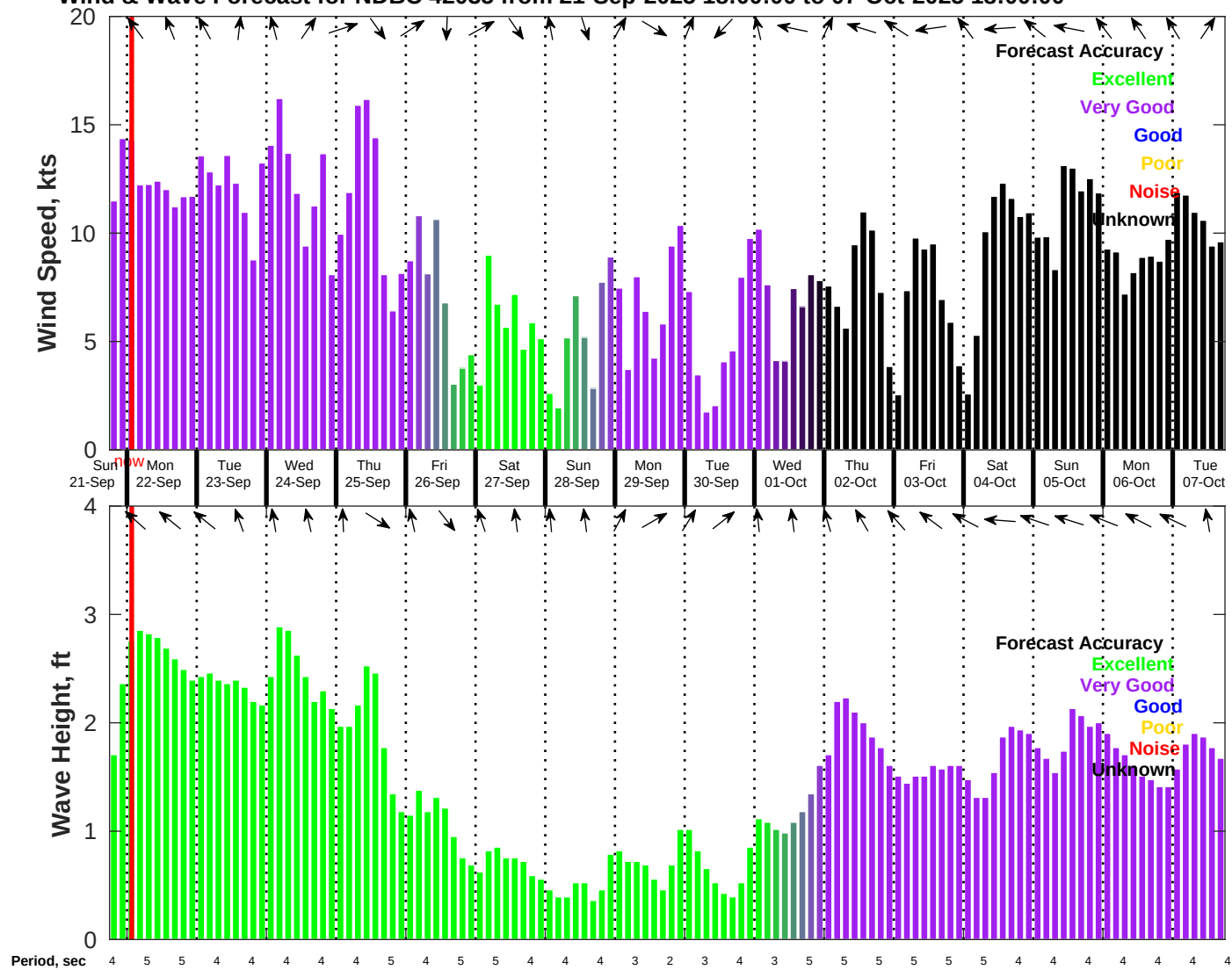
Wind & Wave Forecast for NDBC 42035 from 21-Sep-2025 18:00:00 to 07-Oct-2025 18:00:00
