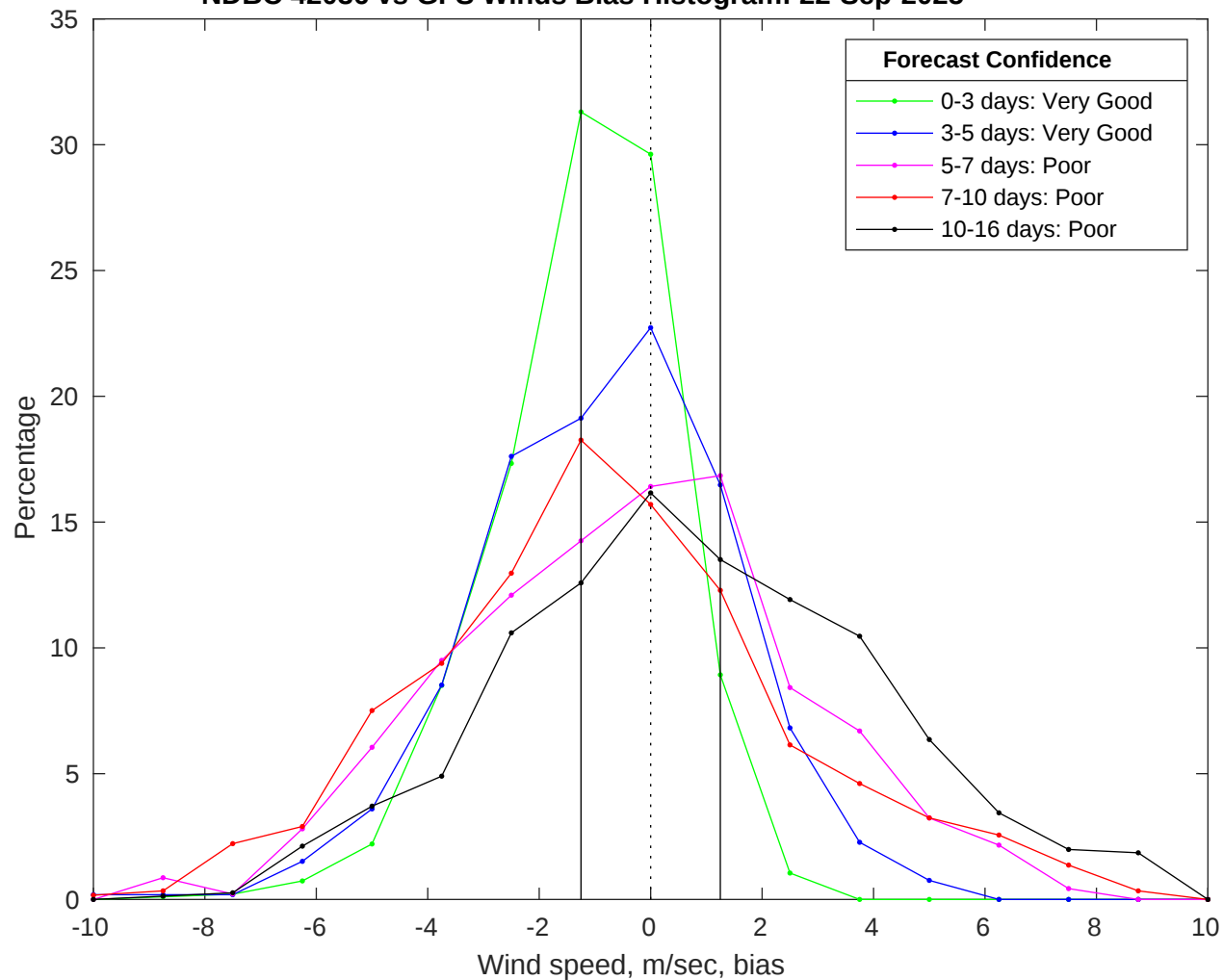
NDBC 42036 vs GFS Winds Bias Histogram: 22-Sep-2025
