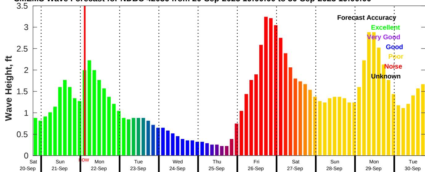
CMEMS Wave Forecast for NDBC 42036 from 20-Sep-2025 19:00:00 to 30-Sep-2025 19:00:00
