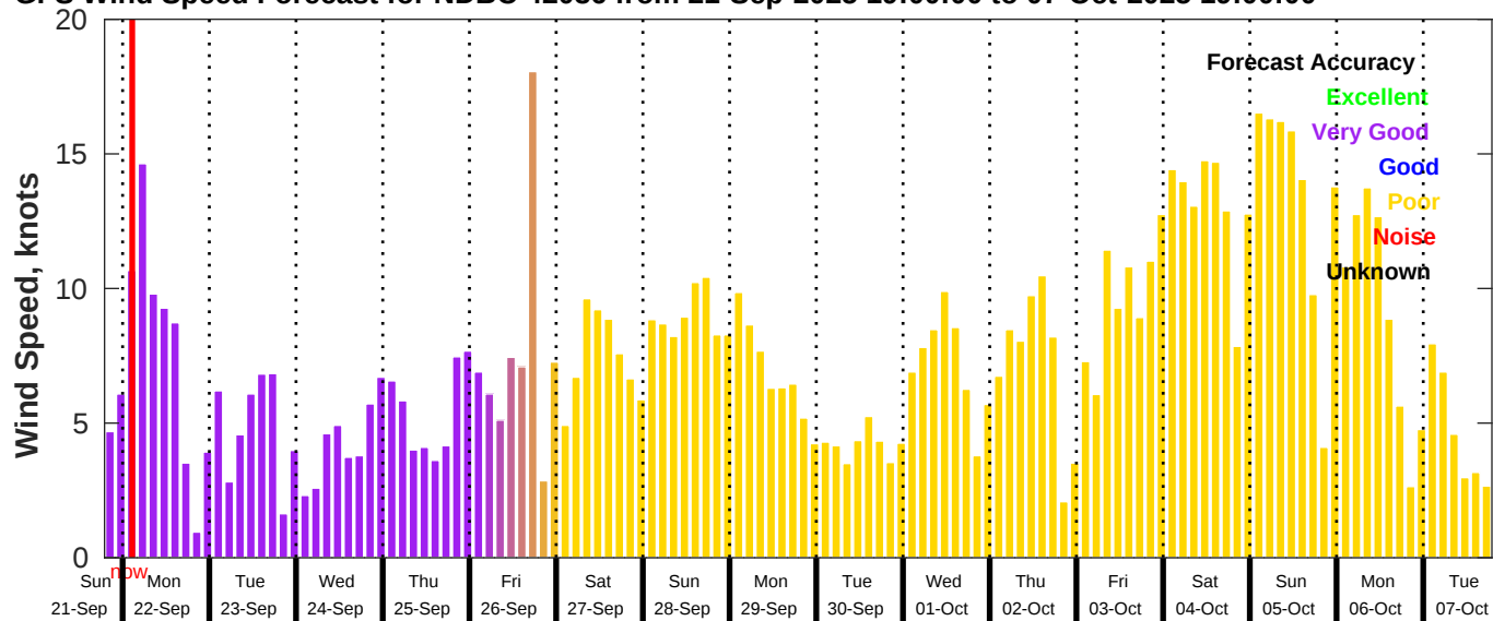
GFS Wind Speed Forecast for NDBC 42036 from 21-Sep-2025 19:00:00 to 07-Oct-2025 19:00:00
