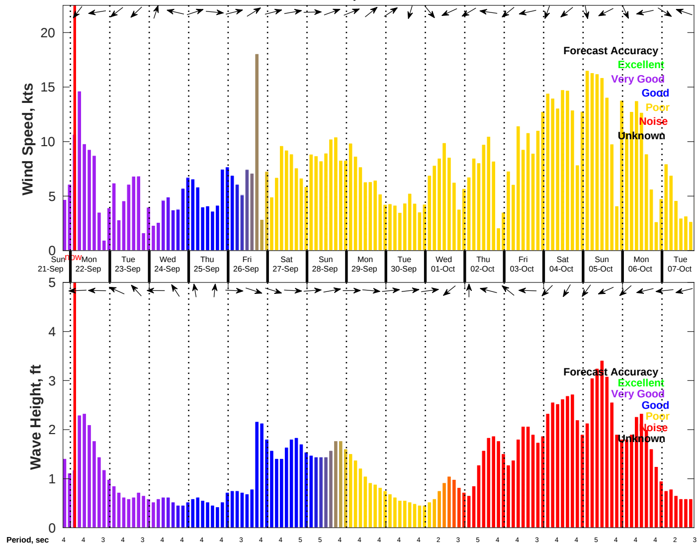
Wind & Wave Forecast for NDBC 42036 from 21-Sep-2025 19:00:00 to 07-Oct-2025 19:00:00
