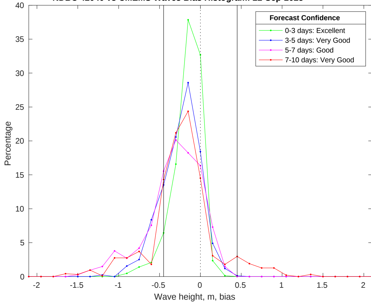
NDBC 42040 vs CMEMS Waves Bias Histogram: 22-Sep-2025
