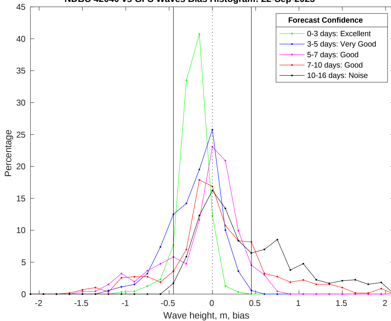
NDBC 42040 vs GFS Waves Bias Histogram: 22-Sep-2025
