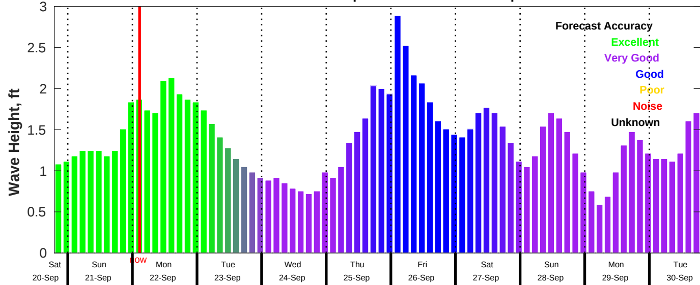
CMEMS Wave Forecast for NDBC 42040 from 20-Sep-2025 19:00:00 to 30-Sep-2025 19:00:00
