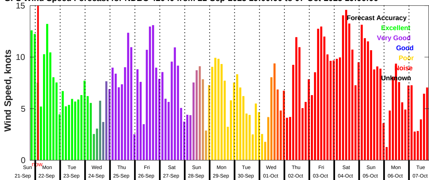
GFS Wind Speed Forecast for NDBC 42040 from 21-Sep-2025 19:00:00 to 07-Oct-2025 19:00:00
