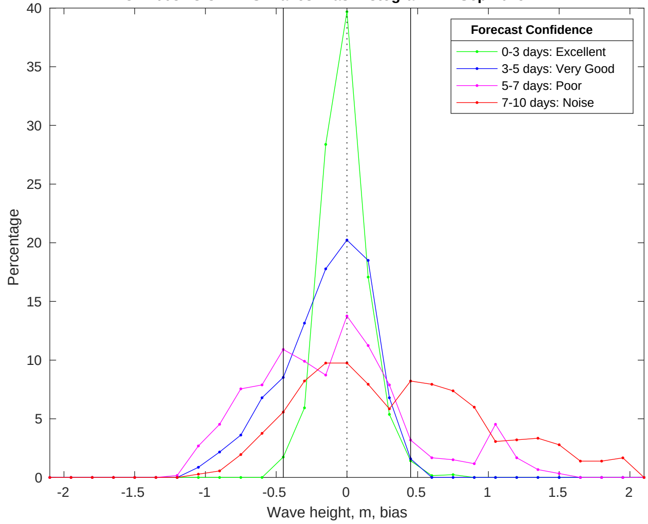
NDBC 44008 vs CMEMS Waves Bias Histogram: 22-Sep-2025
