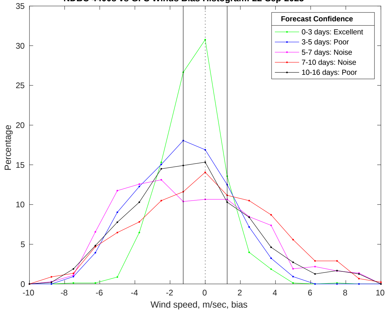
NDBC 44008 vs GFS Winds Bias Histogram: 22-Sep-2025
