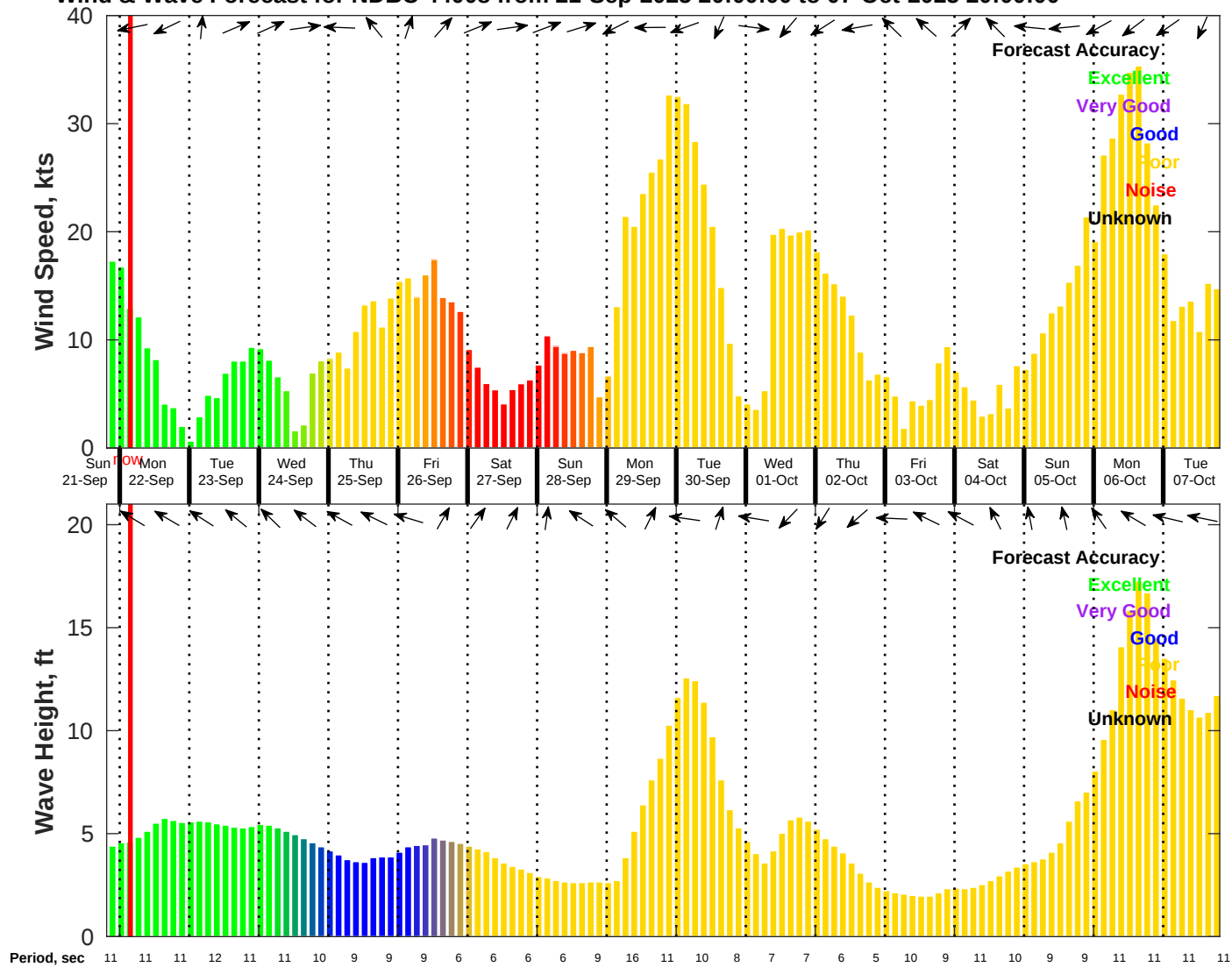
Wind & Wave Forecast for NDBC 44008 from 21-Sep-2025 20:00:00 to 07-Oct-2025 20:00:00
