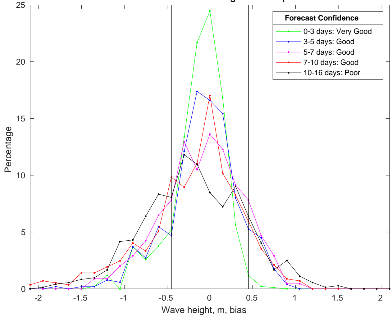
NDBC 46011 vs GFS Waves Bias Histogram: 22-Sep-2025
