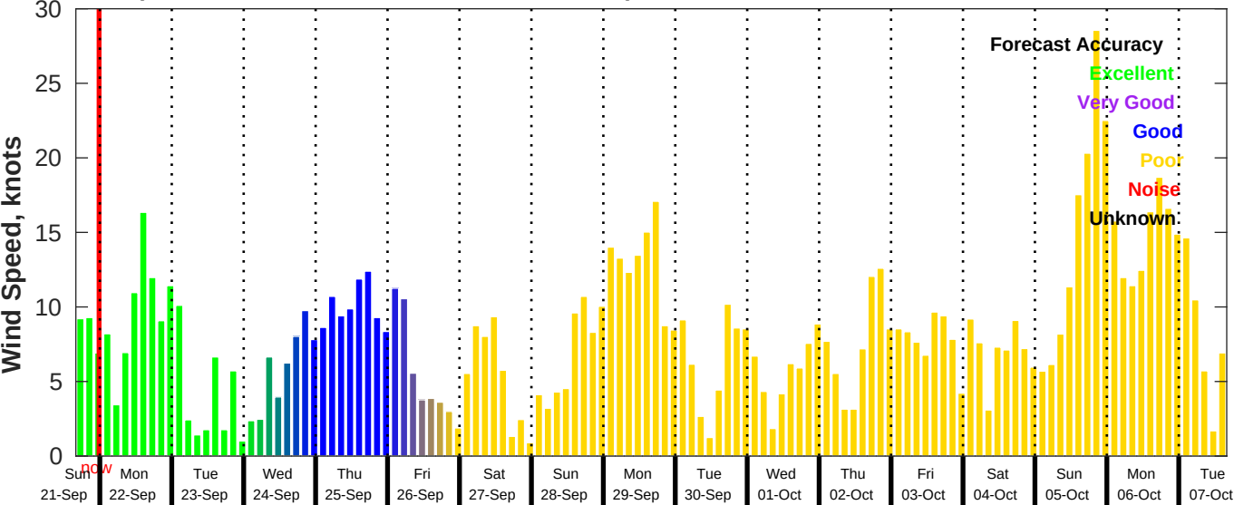
GFS Wind Speed Forecast for NDBC 46011 from 21-Sep-2025 16:00:00 to 07-Oct-2025 16:00:00
