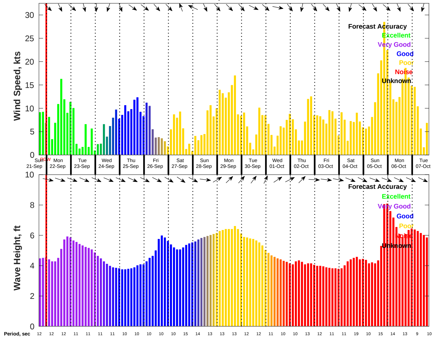
Wind & Wave Forecast for NDBC 46011 from 21-Sep-2025 16:00:00 to 07-Oct-2025 16:00:00
