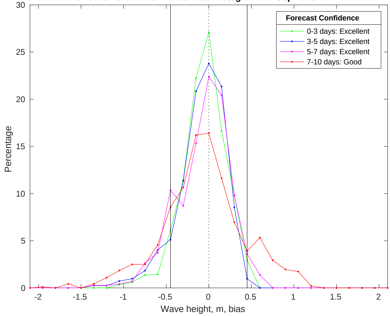
NDBC 46028 vs CMEMS Waves Bias Histogram: 22-Sep-2025
