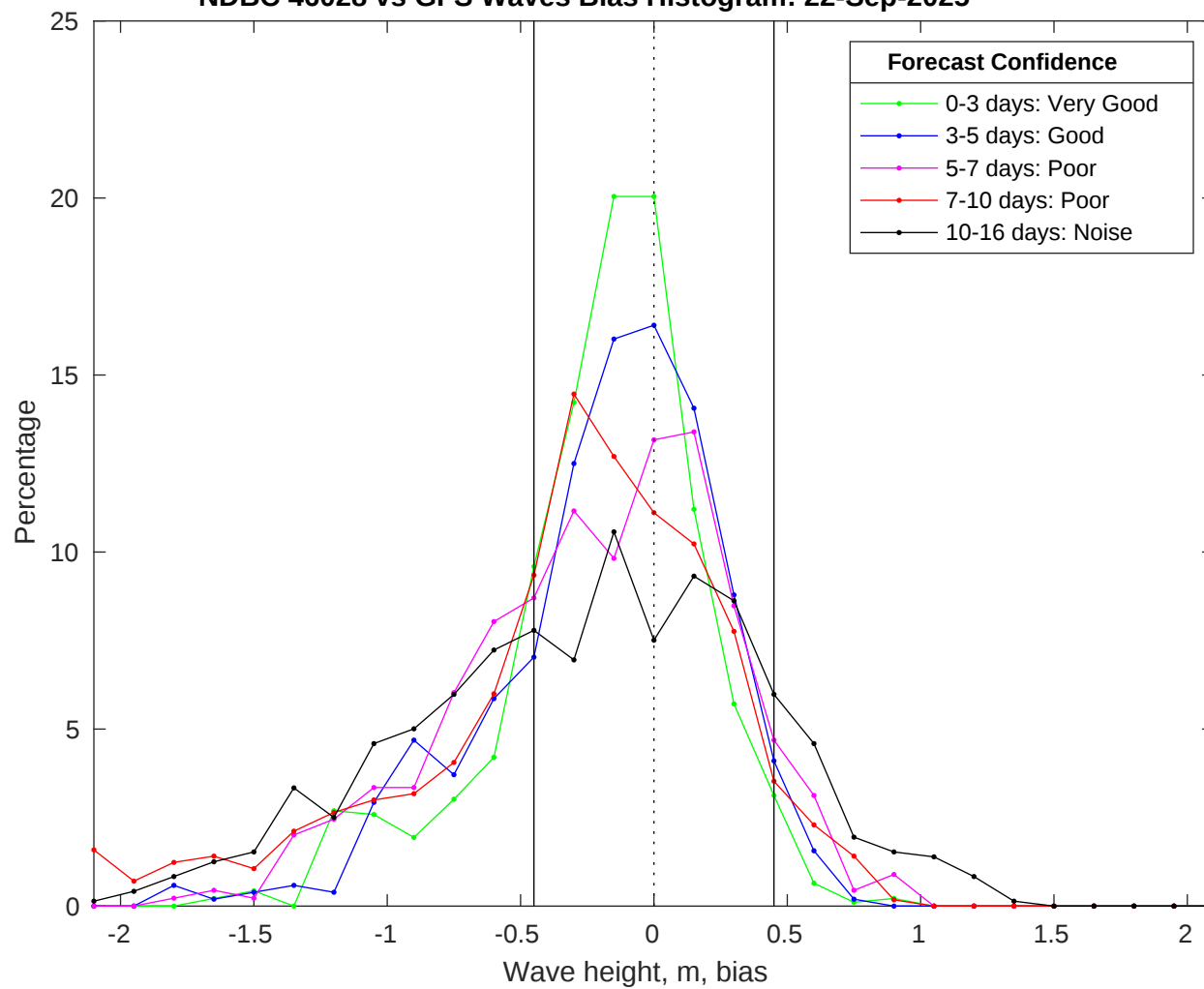
NDBC 46028 vs GFS Waves Bias Histogram: 22-Sep-2025
